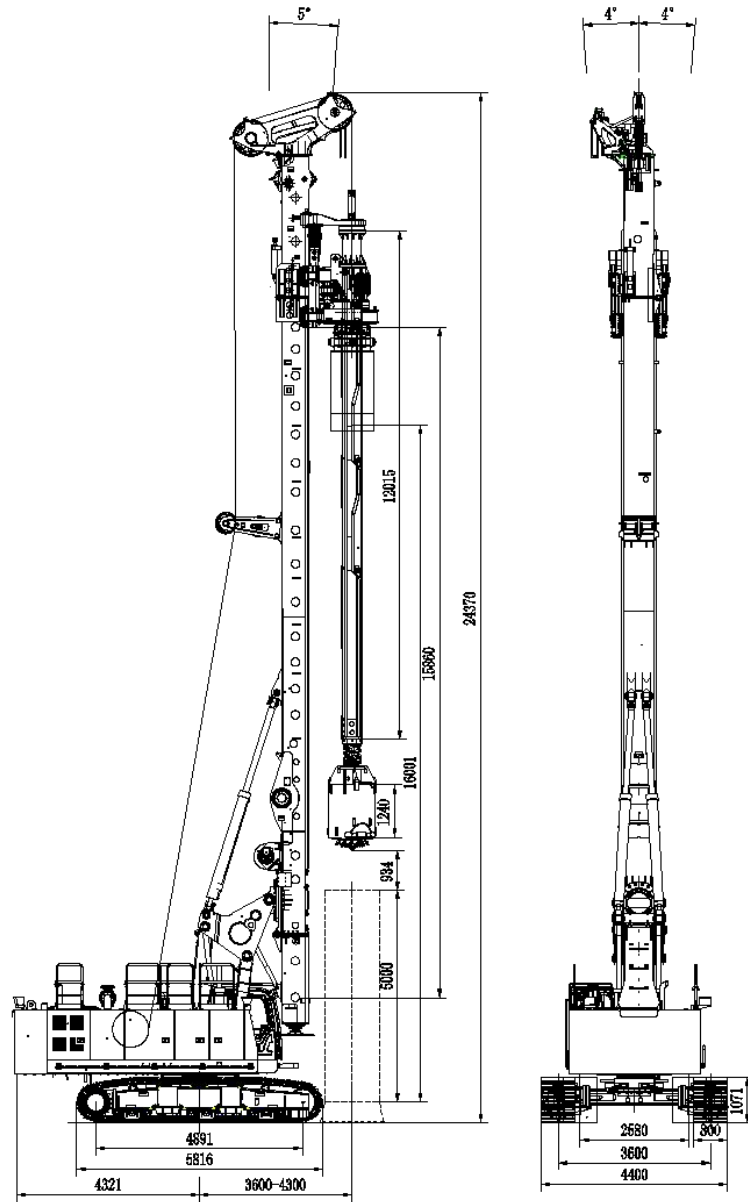
护筒跟进 Cased Kelly Drilling
